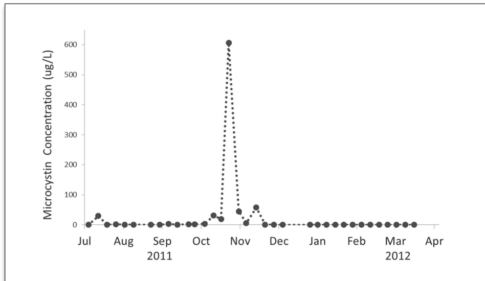
Figure 1. Microcystins
